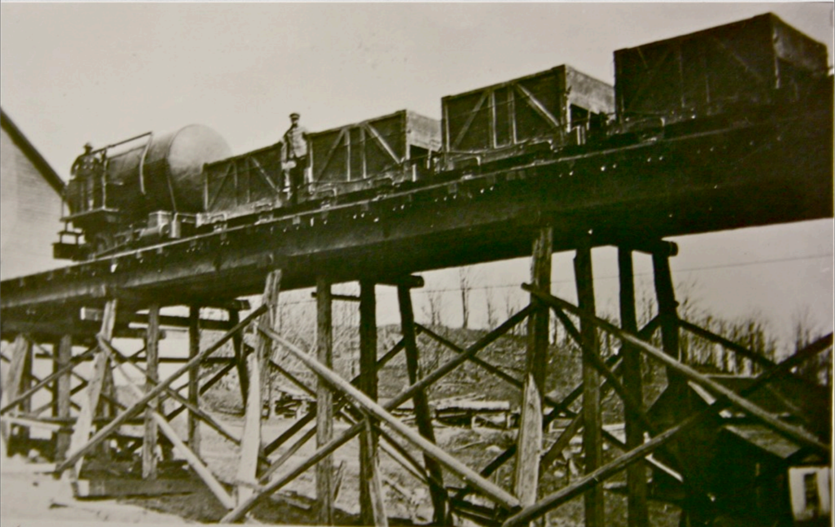
49" gauge rock cars at Atlantic mine, compressed air loco
